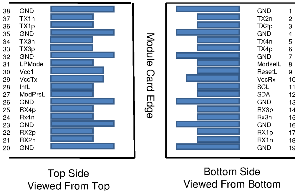
Figure 8: QSFP+ Pin Map
