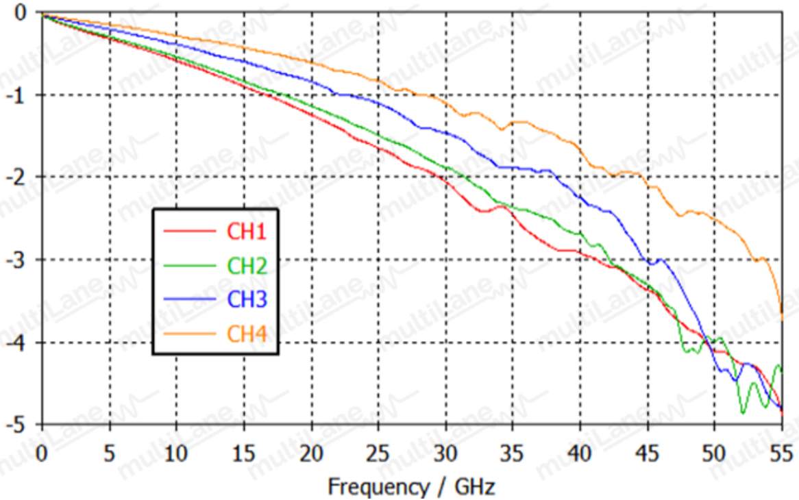
Figure 7: Insertion Loss Graph
